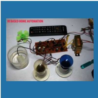
IR Remote Based Home Automation
