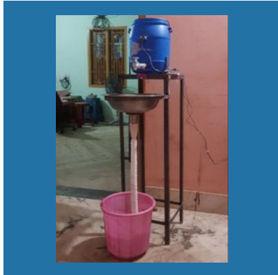
Automatic Water Tap Control Model
