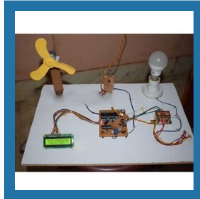
Automatic Room Temp Controller Model
